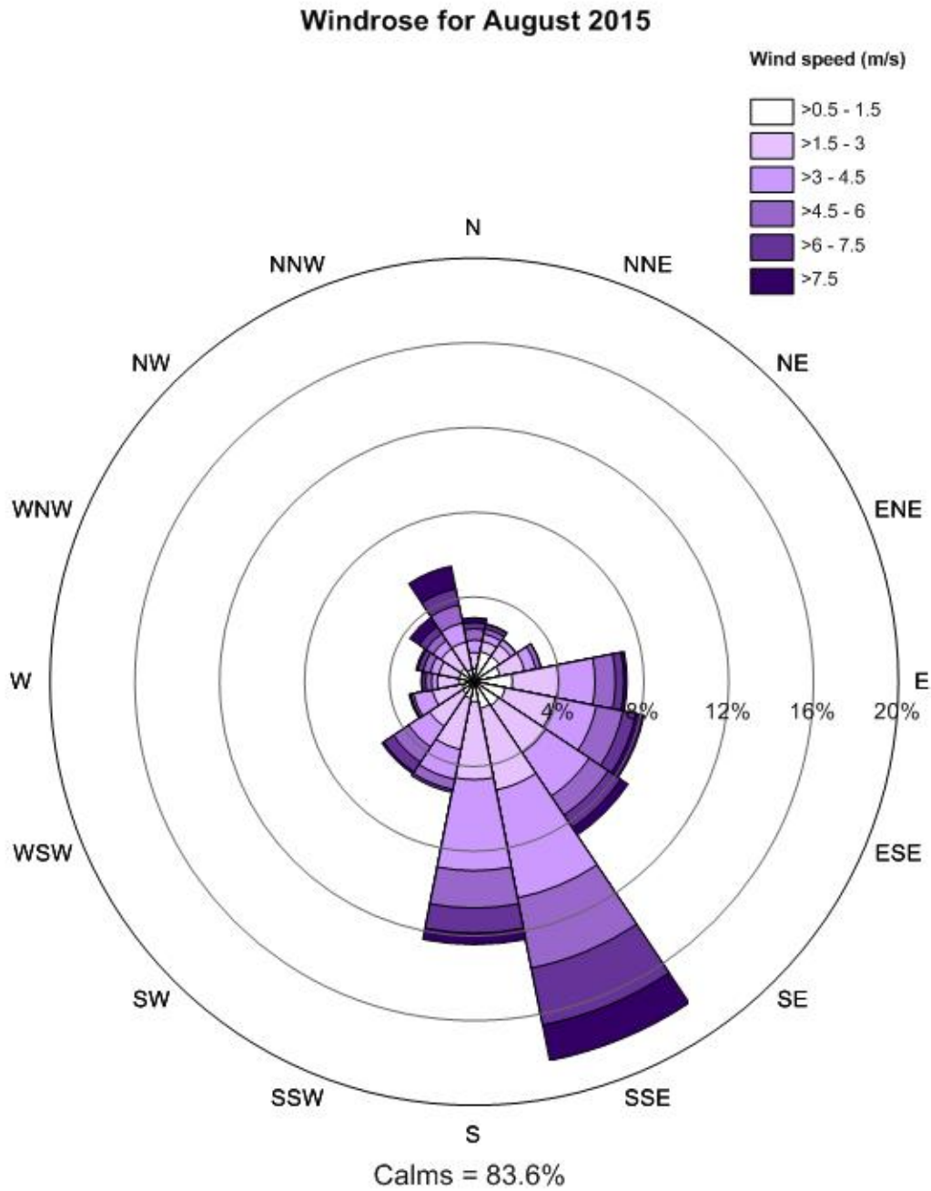
■ Figure 2 August 2015 Windrose, Blacktown International Sportspark Meteorological station
