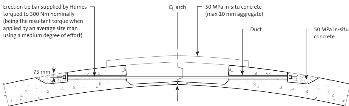
Figure 8 – Arch-to-arch tie rod detail
