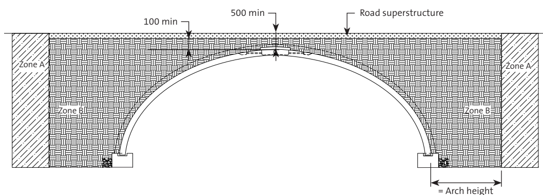
Figure 18 – Low level fills (recommended for overfill up to 500 mm)
