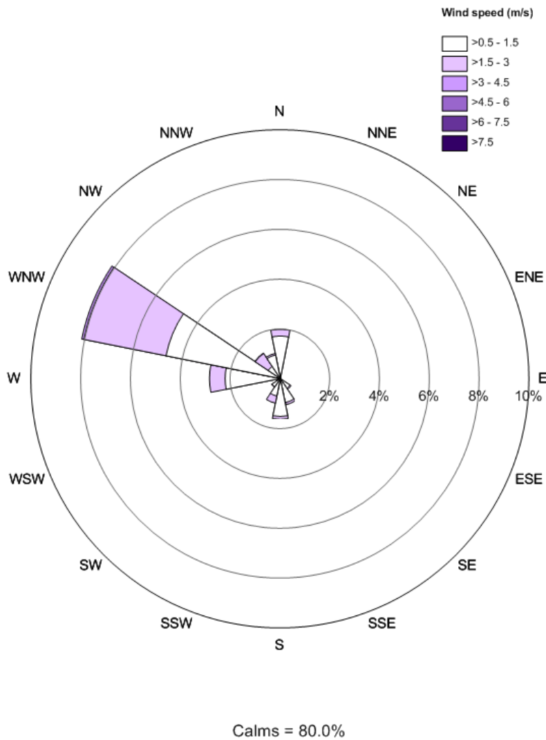
■ Figure 2 July 2014 Windrose, Blacktown International Sportspark Meteorological station
